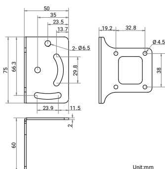
Installation Bracket:
