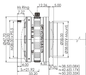
7.OPT-VCT50/2.8-0.17X
