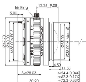
8.OPT-VCT60/4.0-0.17X
