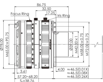
5.OPT-MCT40/4.5-0.08X
