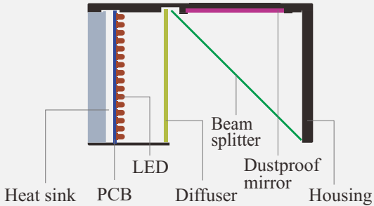
Section Structure Drawing
