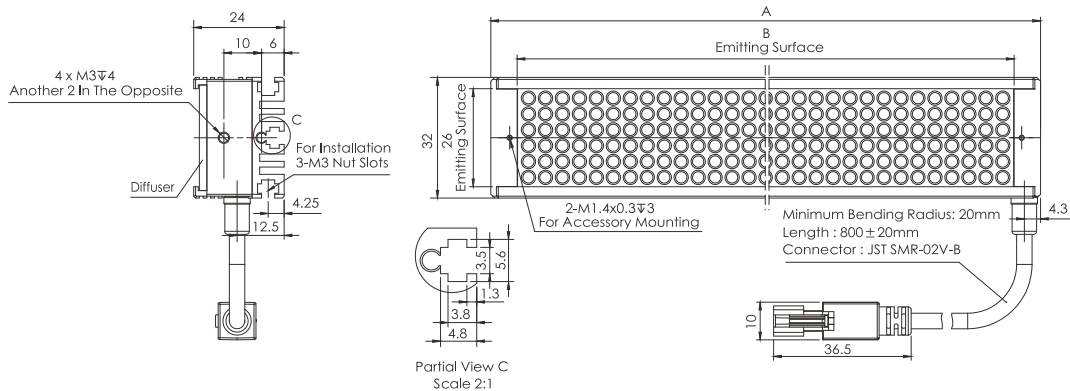
Dimensions (mm)
