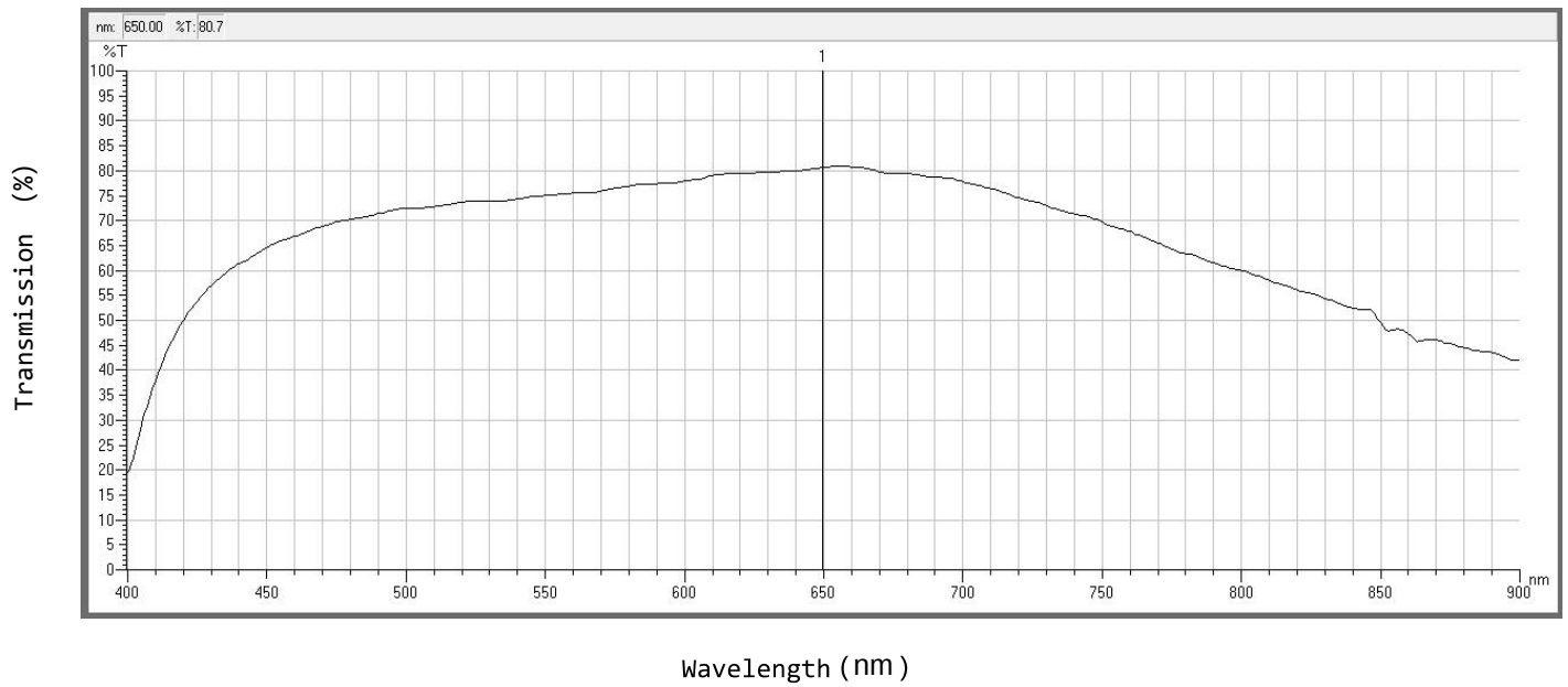
Transmission vs. Wavelength
