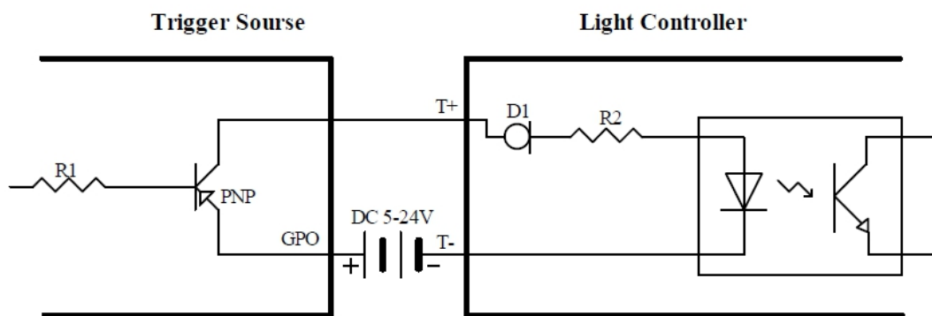
Trig Input Circuit For PNP Type Trigger
