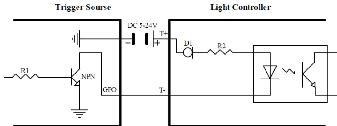
Trig Input Circuit For NPN Type Trigger
