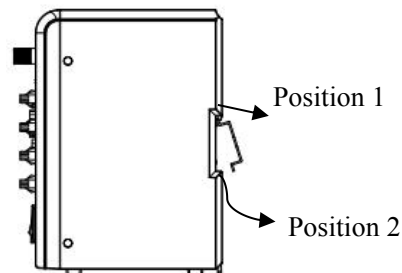
Figure 1 Mounting steps
