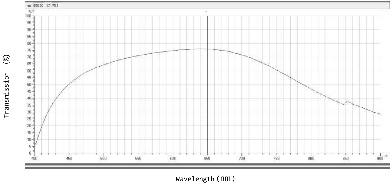
Transmission vs. Wavelength
