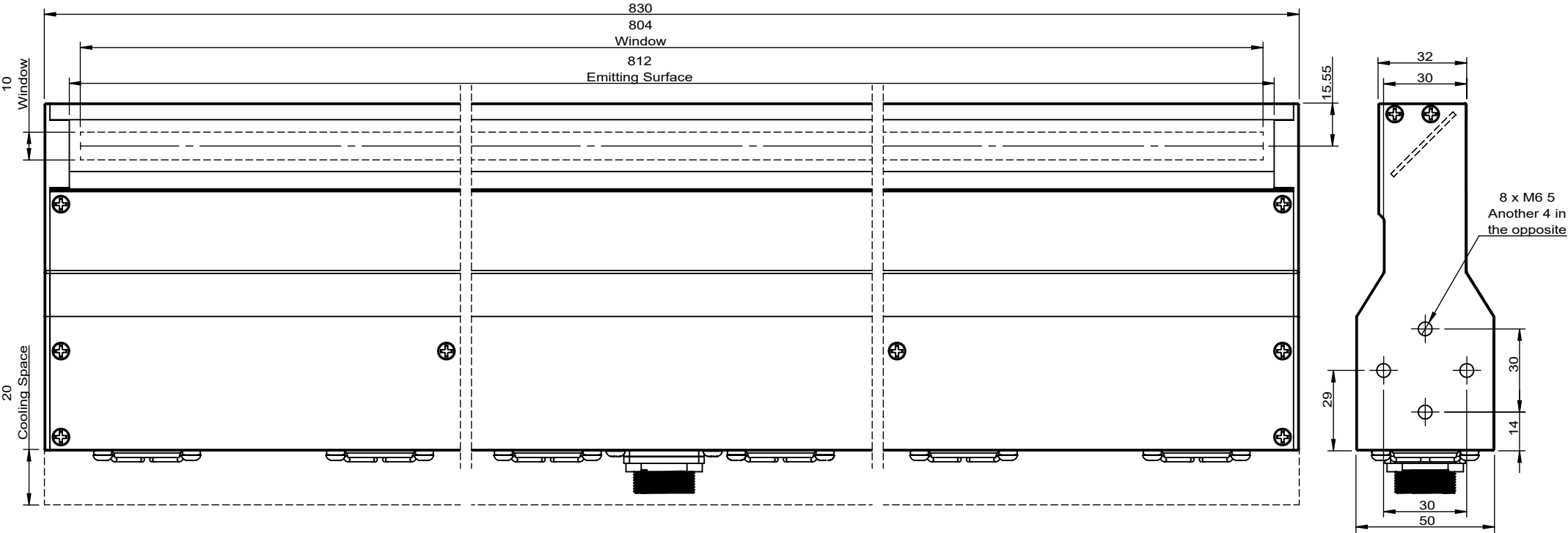
Connector: WS20K6Z
